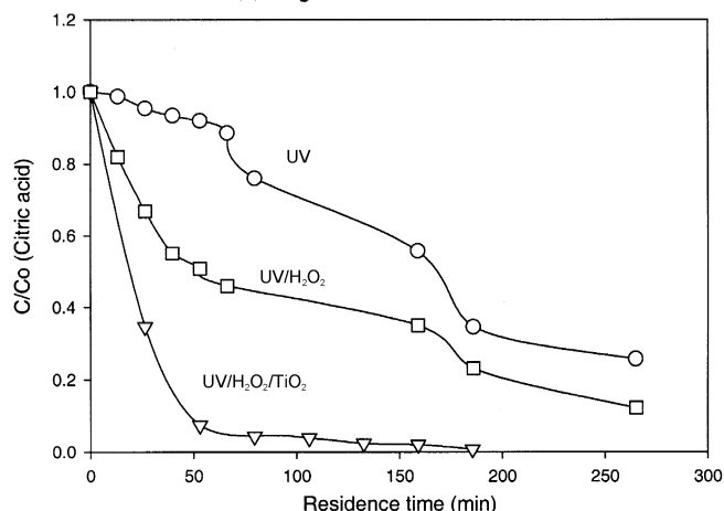
(b) Degradation of citric acid
