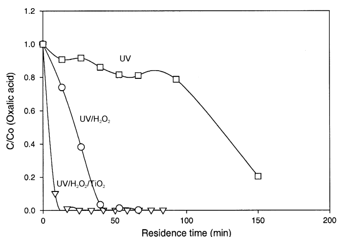
(a) Degradation of oxalic acid
